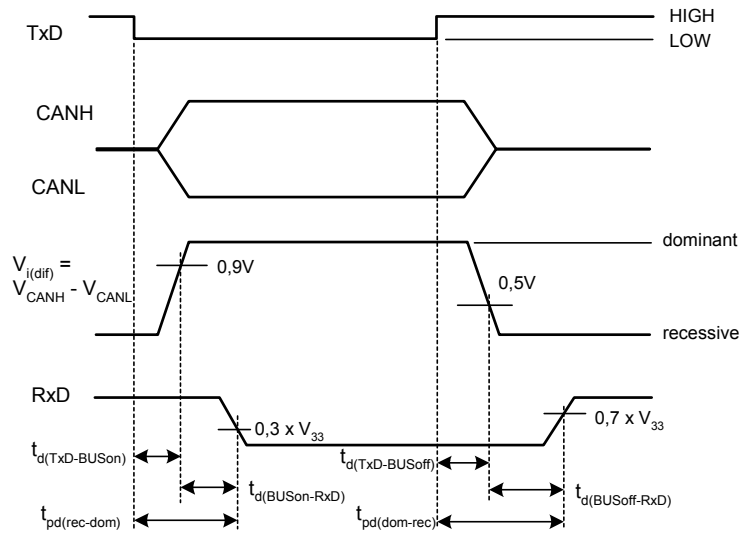
Figure 7: Timing Diagram for AC Characteristics
