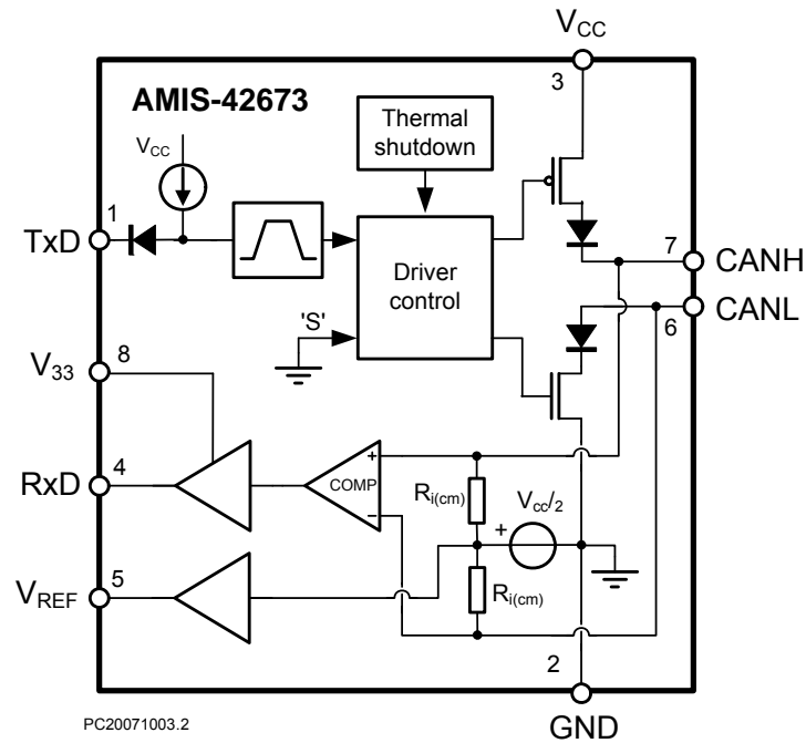
Figure 1: Block Diagram
