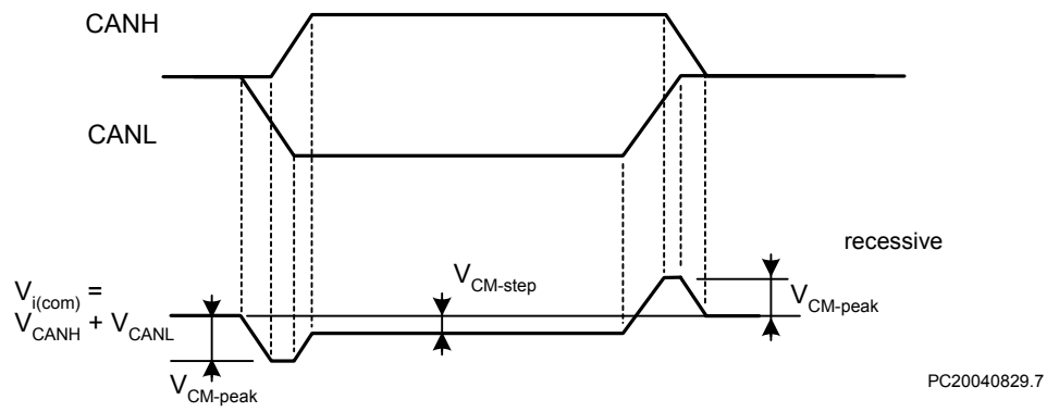
Figure 9: Common-mode Voltage Peaks (see measurement set-up Figure 8)
